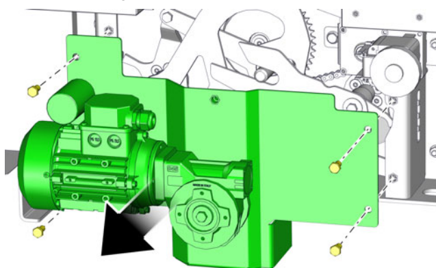
Sl. 8-13: Pogon
