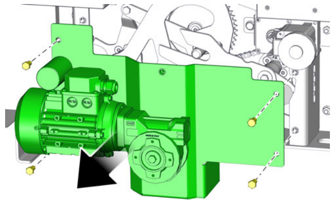
Sl. 8-13: Pogon
